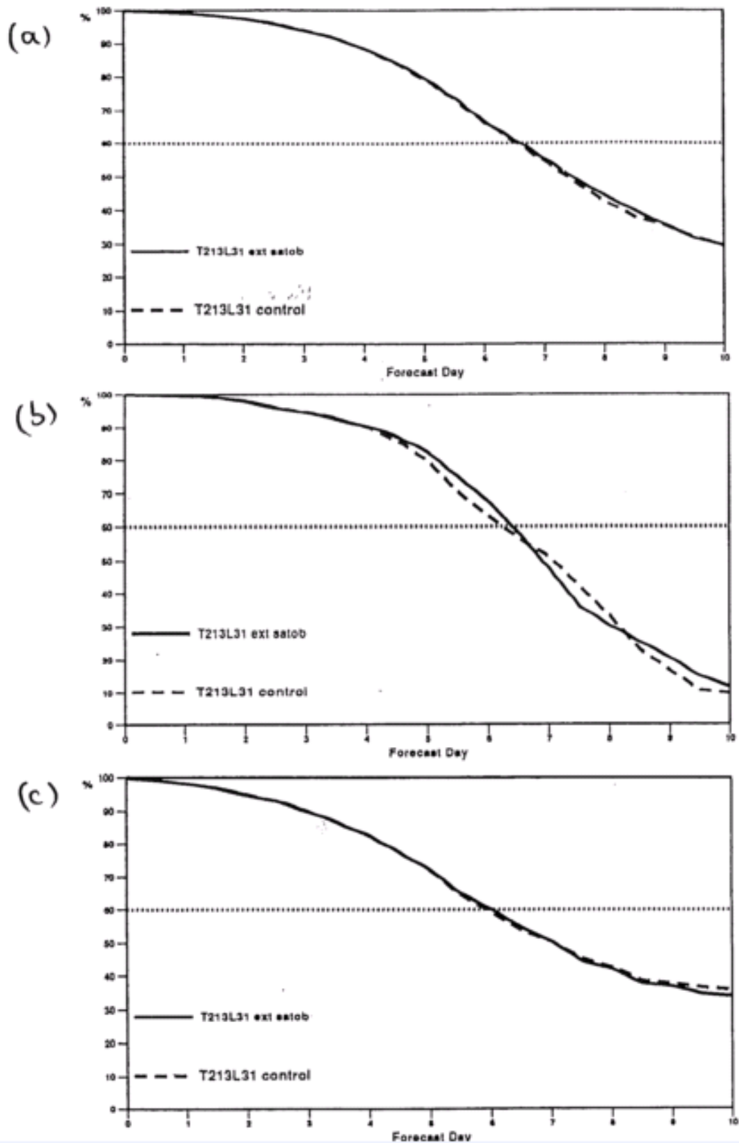
Fig. 8. Anomaly correlation for examining the impact of modifying the current operation blacking in order that GMS and GOES are treated the same as METEOSAT. The solid line is the modified blacklist experiment and the dashed the than current operations. (a) Northern hemisphere, (b) Results for the european area, (c) Southern hemisphere.
