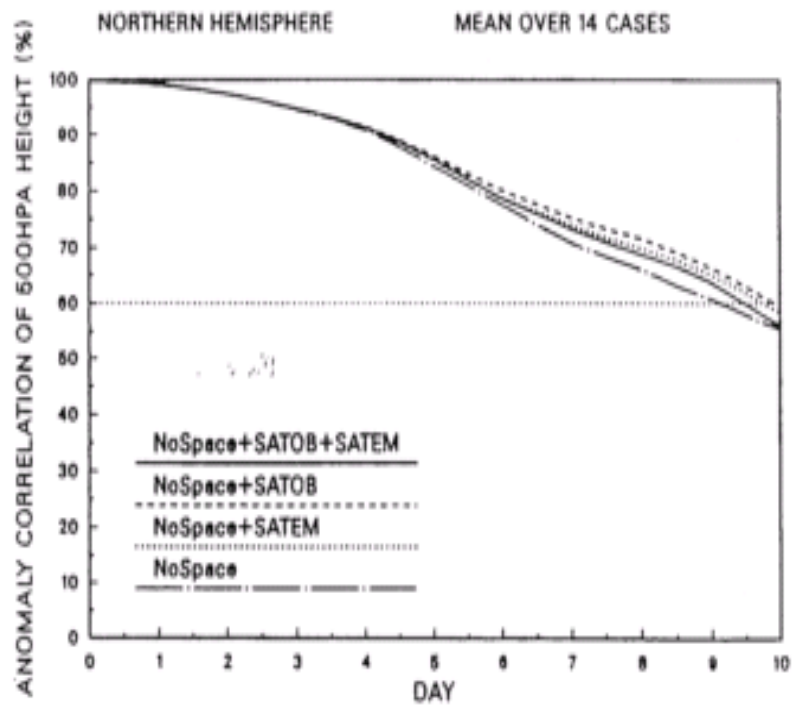
Fig. 7. Northern Hemisphere extra-tropics anomaly correlations of 500hPa for a two week period in February 1989. Impact of space observing systems (SATEMS, SATOBS and the combination).
