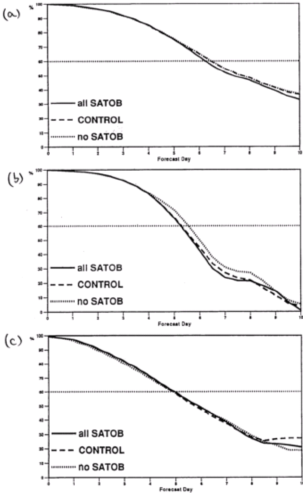
Fig.9. Anomaly correlation for examining : (i) the impact of modifying the current operation blacking in order that GMS and GOES are treated the same as METEOSAT. The solid line is the modified blacklist experiment and the dashed the than current operations, (ii) the impact of removing all satobs from the assimilation (dotted). (a) Northern hemisphere, (b) Results for the european area, (c) Southern hemisphere.
