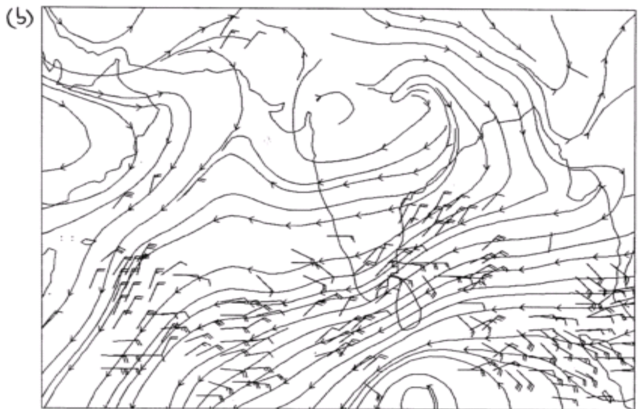
Fig. 4 A comparison between INSAT SATOBs, ship winds and ECMWF analysis. (a) Ship observations plotted with 1000 hPa streamlines. (b) INSAT SATOBs observations plotted with 850 hPa streamlines.
