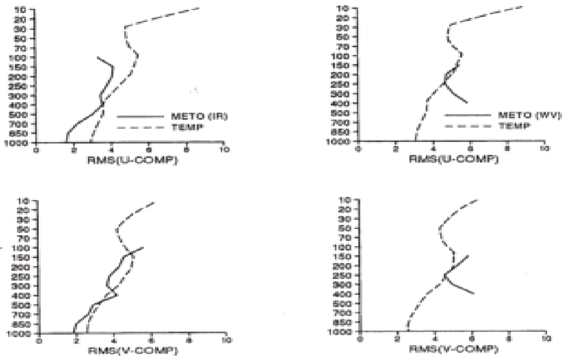
Fig. 6. Same as Fig. 4 for the tropical belt (20°N to 20°S).
