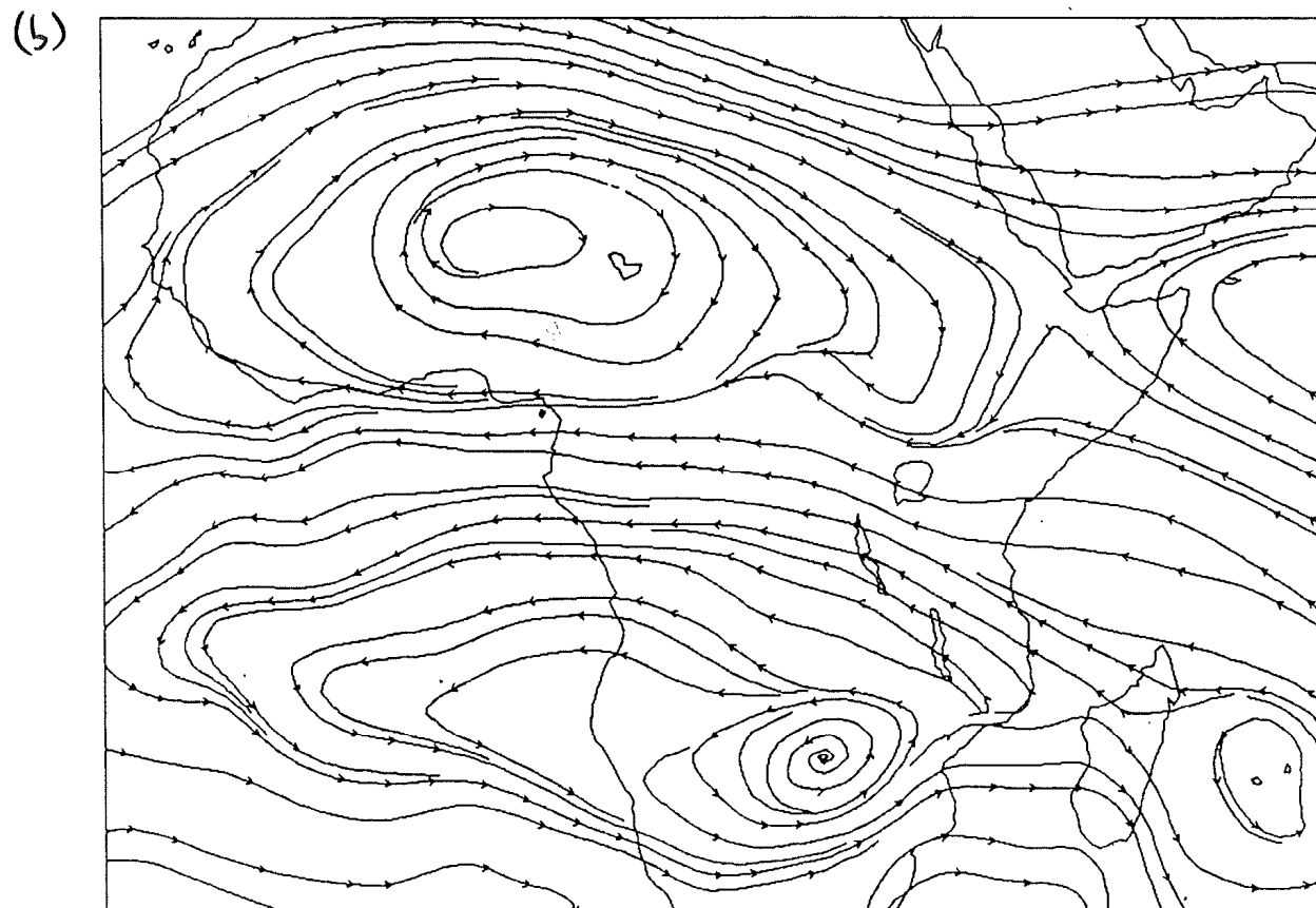
Fig. 10. Wind stream lines for the 12 UTC 6/3/1993 ECMWF analysis. (a) 150 hPa, (b) 250 hPa.
