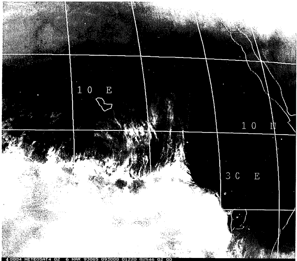
Fig. 12. Meteosat 6.3 micron water vapour channel.
