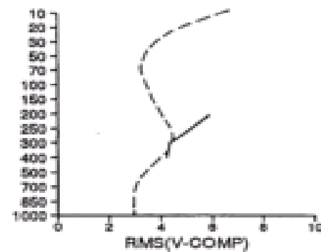
Fig. 5 First Guess differences for radiosondes (dashed) and satobs (solid) but for the Northern Hemisphere (20°N to 50°N).
