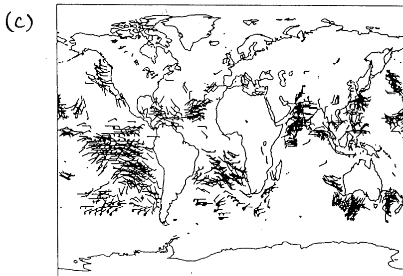
Fig. 2 Data coverage of satobs received operational at ECMWF on the 18 January 94. (a) Upper level satobs from 350 to 100 hPa. (b) Mid level satobs from 811 to 349 hPa. (c) Lower level satobs from 1000 to 800 hPa.
